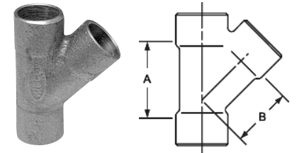
749 ⚠ 45° Y C x C x C – Cast
