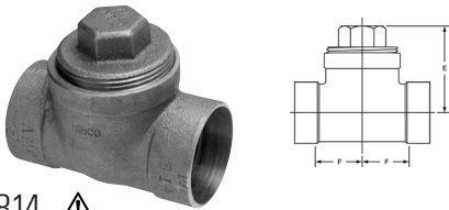
814 \Delta DWV Test Tee C x C x Cleanout w/Plug – Cast
