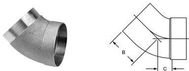
806-2 \Delta DWV 45° Fitting Elbow Ftg x C – Cast
