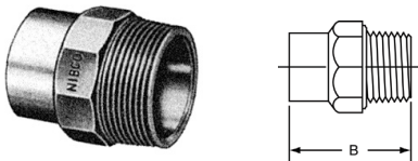
804-2 DWV Fitting Adapter Ftg x M – Cast
