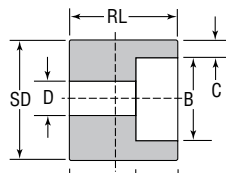
Type 2 - Reducer Insert Fig. 2179
