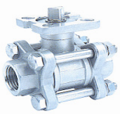
B05 SERIES 3 pc, full port, CF8M body, 316SS ball and stem, CF8M NPT ends, RTFE seats and seals, locking lever handle, ISO direct mount Size ½" to 4" 1000 PSI
