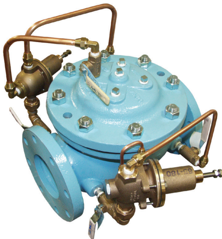
A129 SHOWN WITH OPTIONAL LOW FLOW BYPASS (A129LF)
